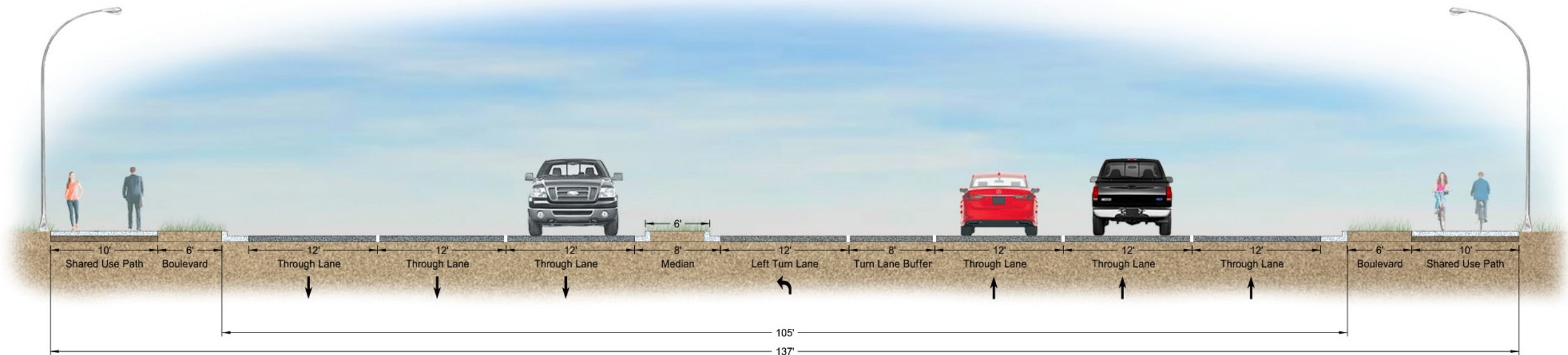
Six-Lane Section With Raised Median and Turn Lanes
