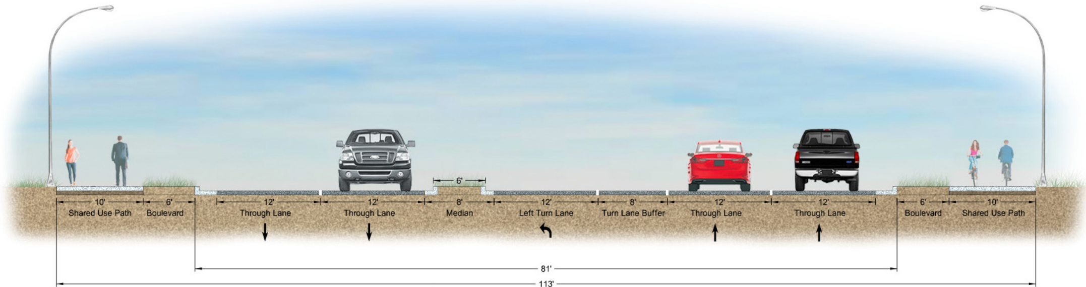
Four-Lane Section With Raised Median and Turn Lanes
